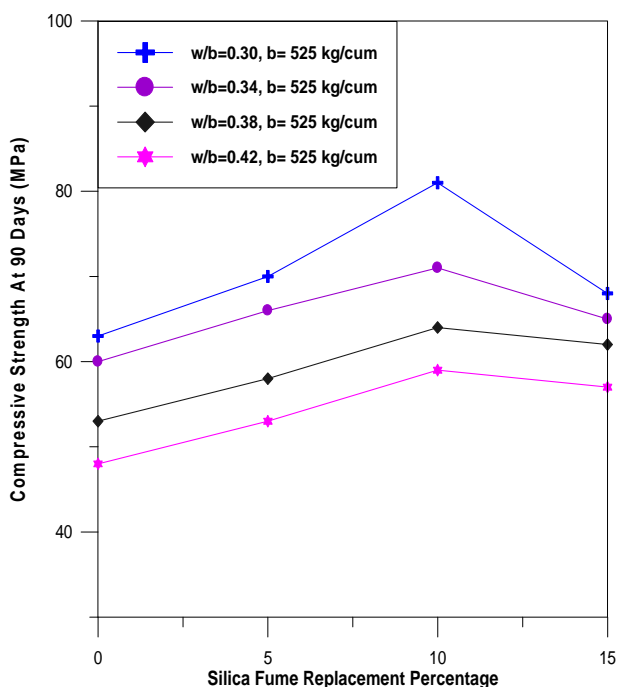
Fig. 3: Compressive Strength at 90 days with Silica Fume Replacement %
