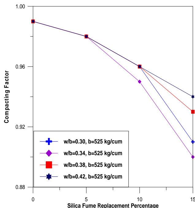
Fig. 1: Variation of Compacting Factor With Silica Fume Replacement Percentage For Different w/b ratios.
