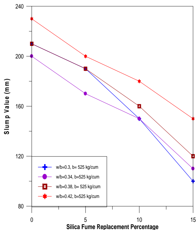
Variation Of Slump With Silica Fume Replacement Percentage For Different w/b ratios.
