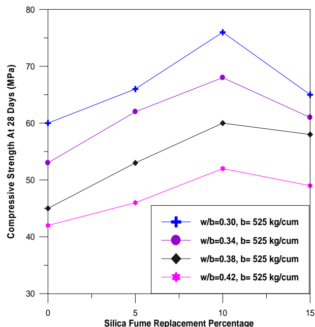
Fig. 2: Compressive Strength at 28 days with Silica Fume Replacement %
